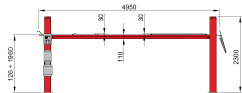
ERCO 4004 BCT LOW PROFILE, RECESSED RUNWAYS FOR WHEEL ALIGNMENT
