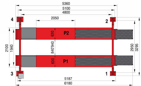
ERCO 4004 BCT LOW PROFILE, RECESSED RUNWAYS FOR WHEEL ALIGNMENT
